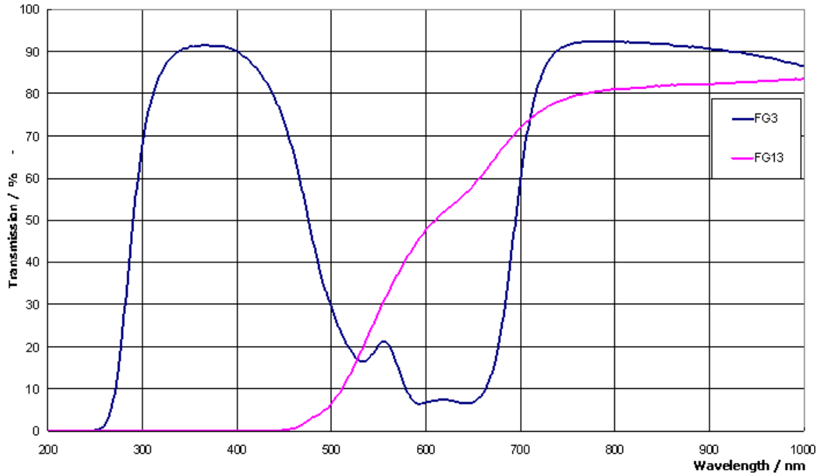
FG - filters, th 3 mm
