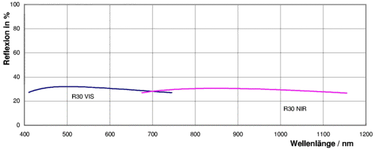
Teller R / T = 50 / 50 +/- 5 , 45° BK7
